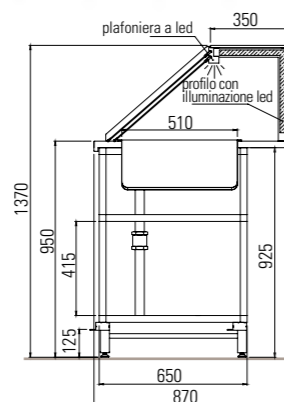
Calda a bagno maria con piano forato Hot water bath with perforated top
